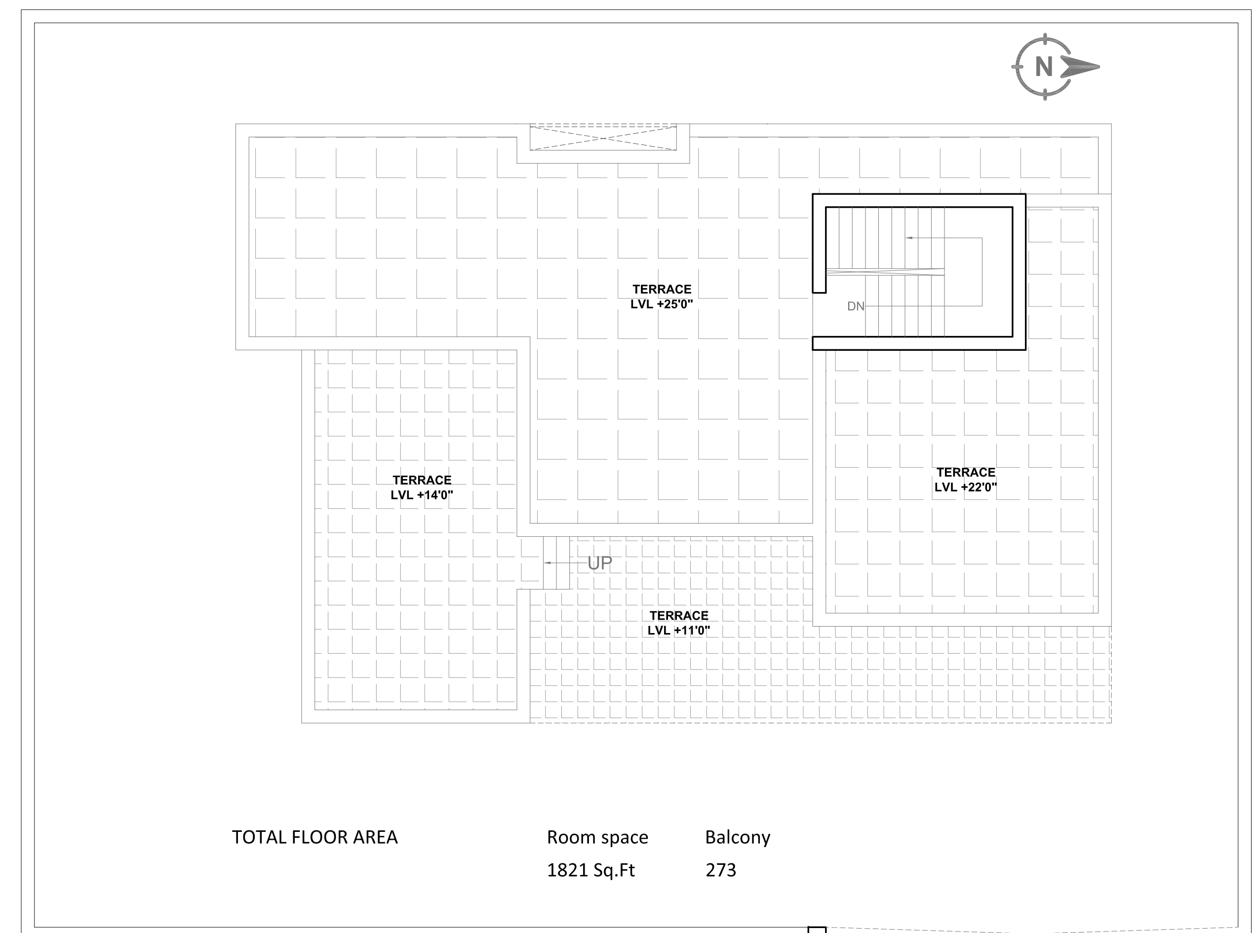
SITE WITH TERRACE FLOOR PLAN (@25'0")
