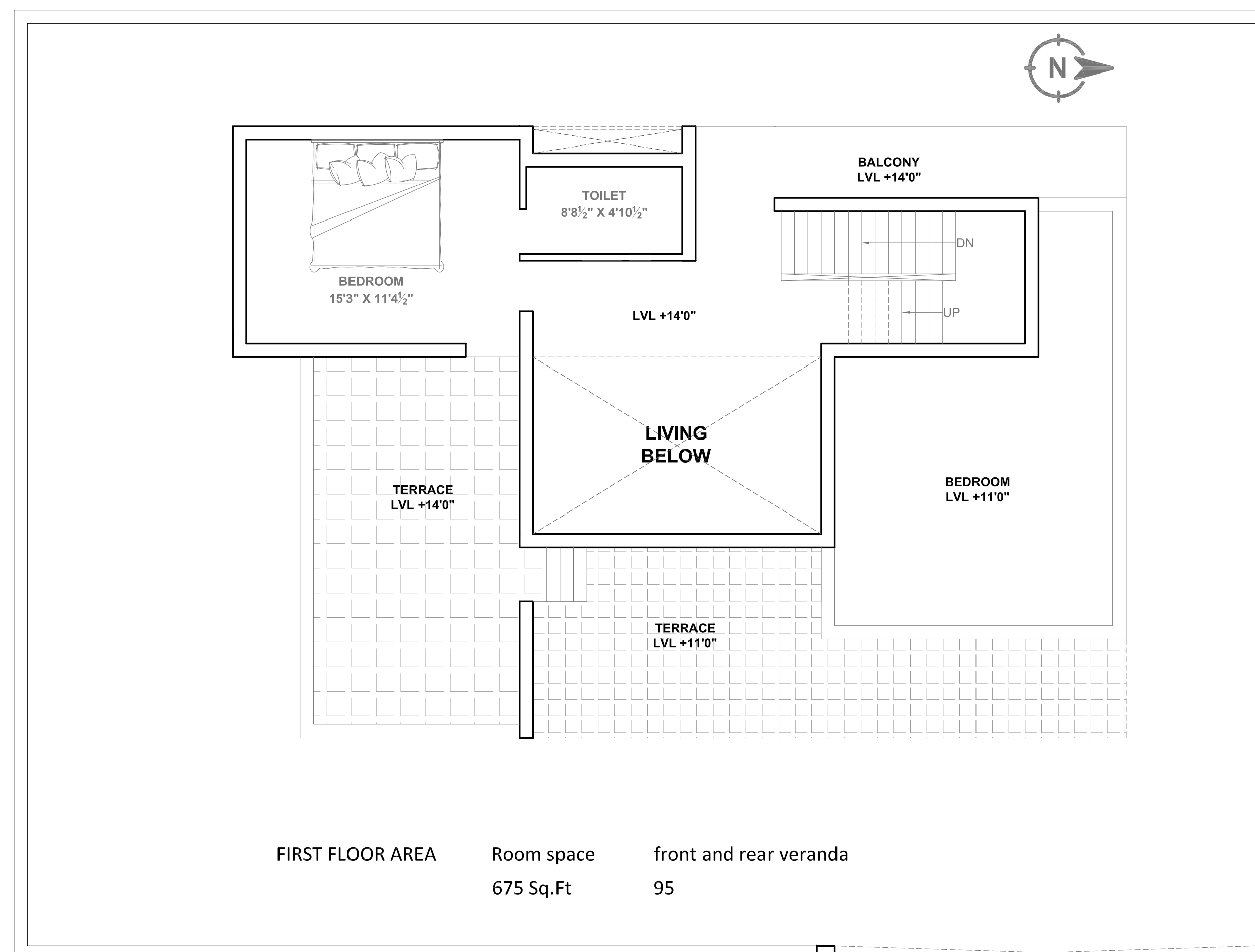
SITE WITH FIRST FLOOR PLAN (@14'0")
