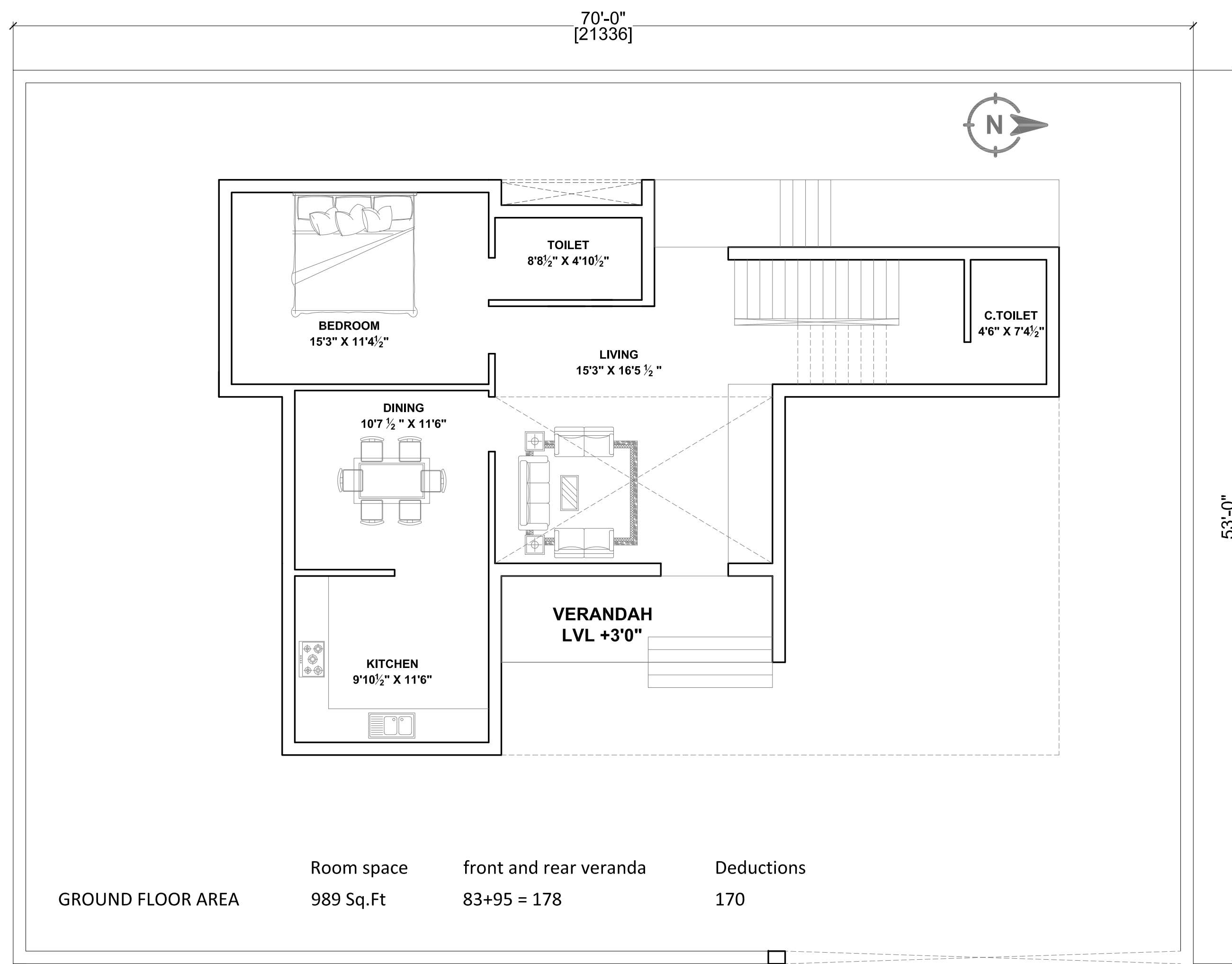
SITE WITH GROUND FLOOR PLAN (@3'0")
